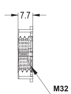
Locknut A
