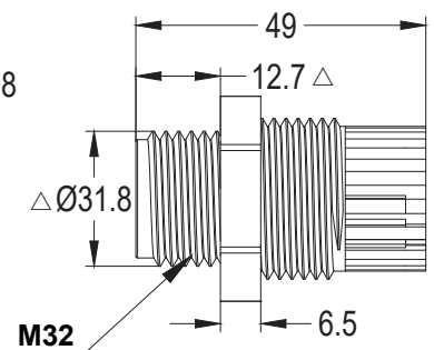
Body C
