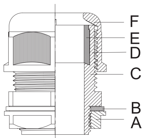
Seal E
