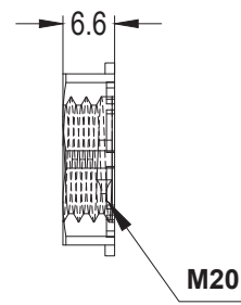
Locknut A
