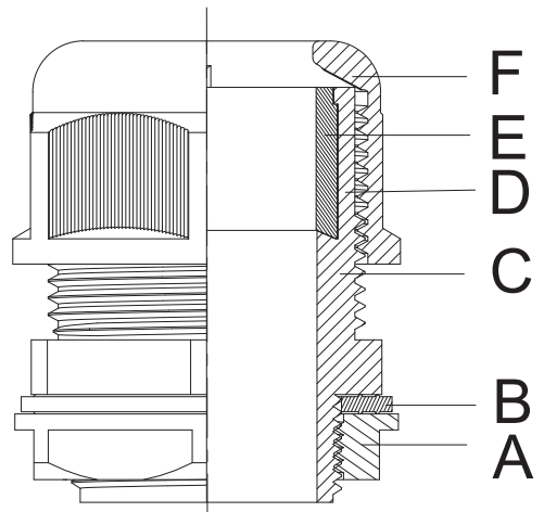
Seal E
