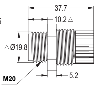
Body C
