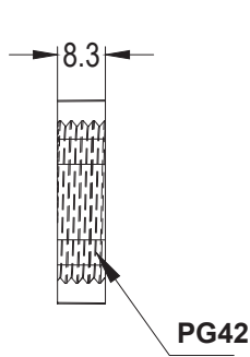
Locknut A
