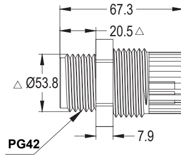
Body C
