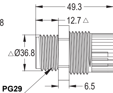
Body C
