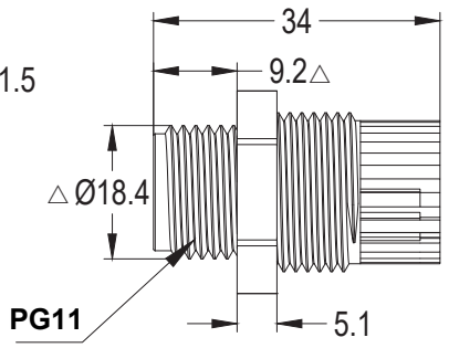
Body C
