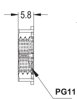
Locknut A
