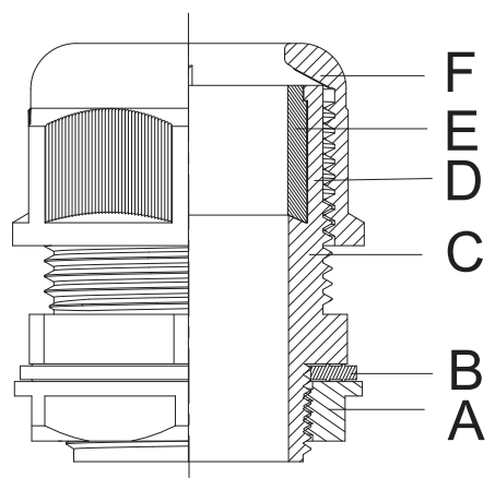
Seal E
