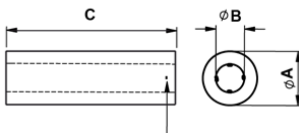
HALTERIPPEN 4x SELF RETAINING RIBS 4x
